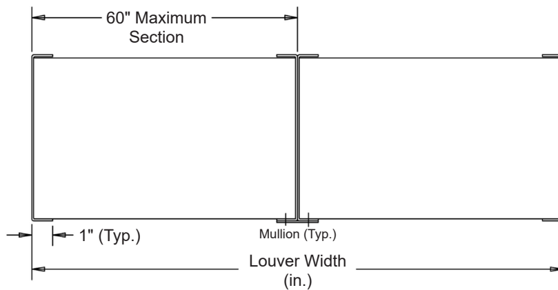
Louver Top View
